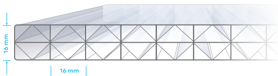
16 mm, 3 layers, X-structure PTS/16/3X
