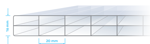
16 mm, 3 layers, rectangular structure PTS/16/3RS
